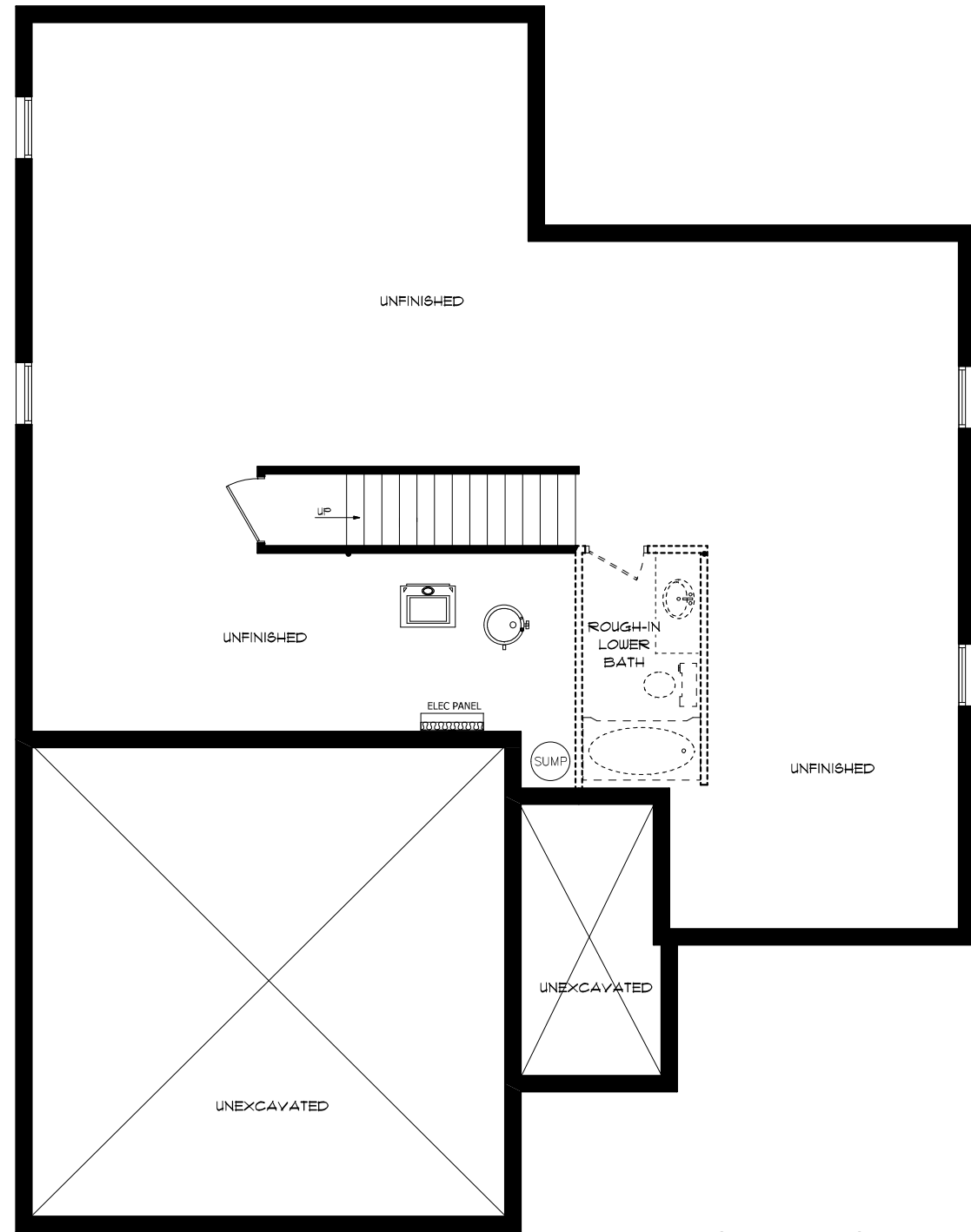
FOUNDATION PLAN
