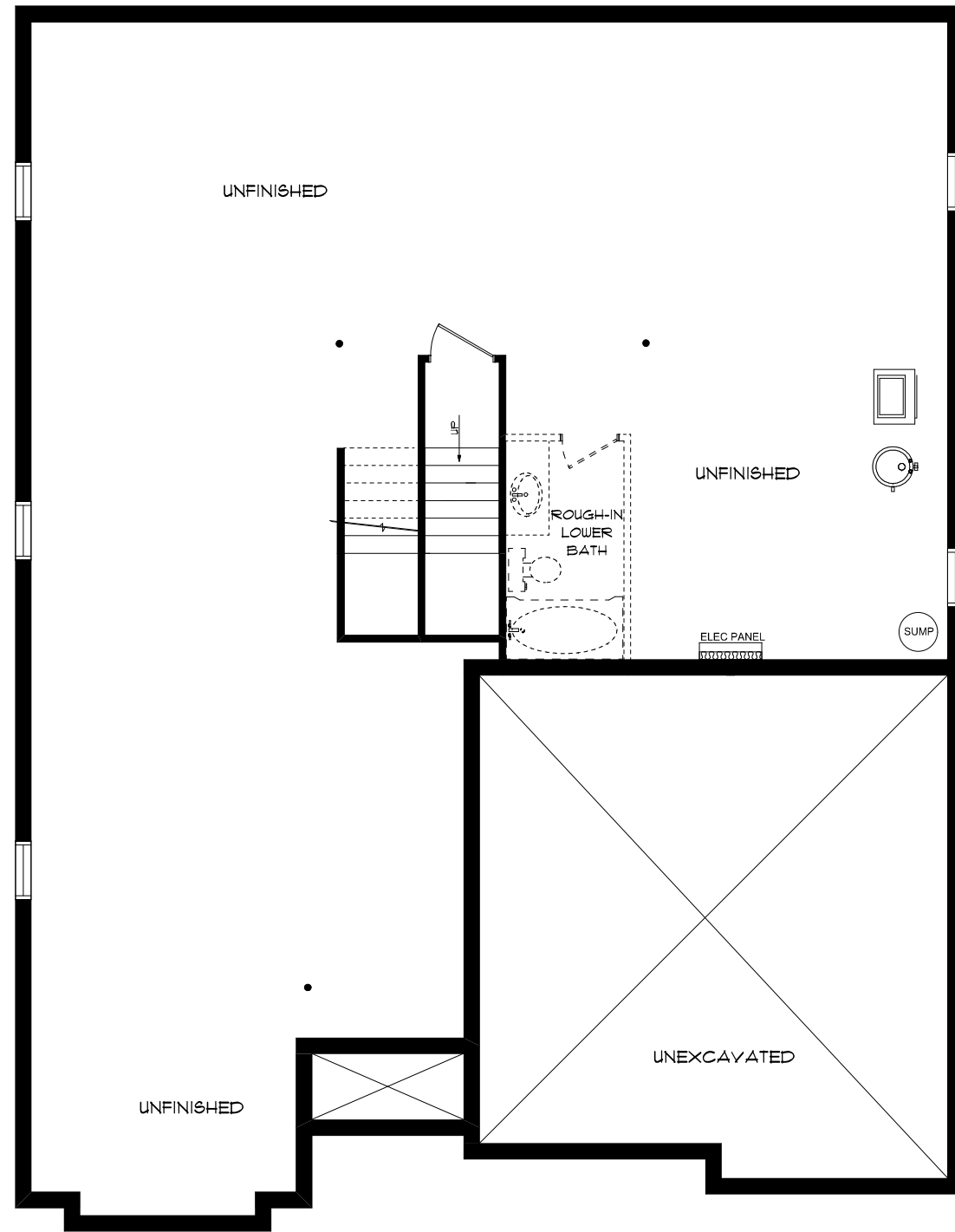
FOUNDATION PLAN
