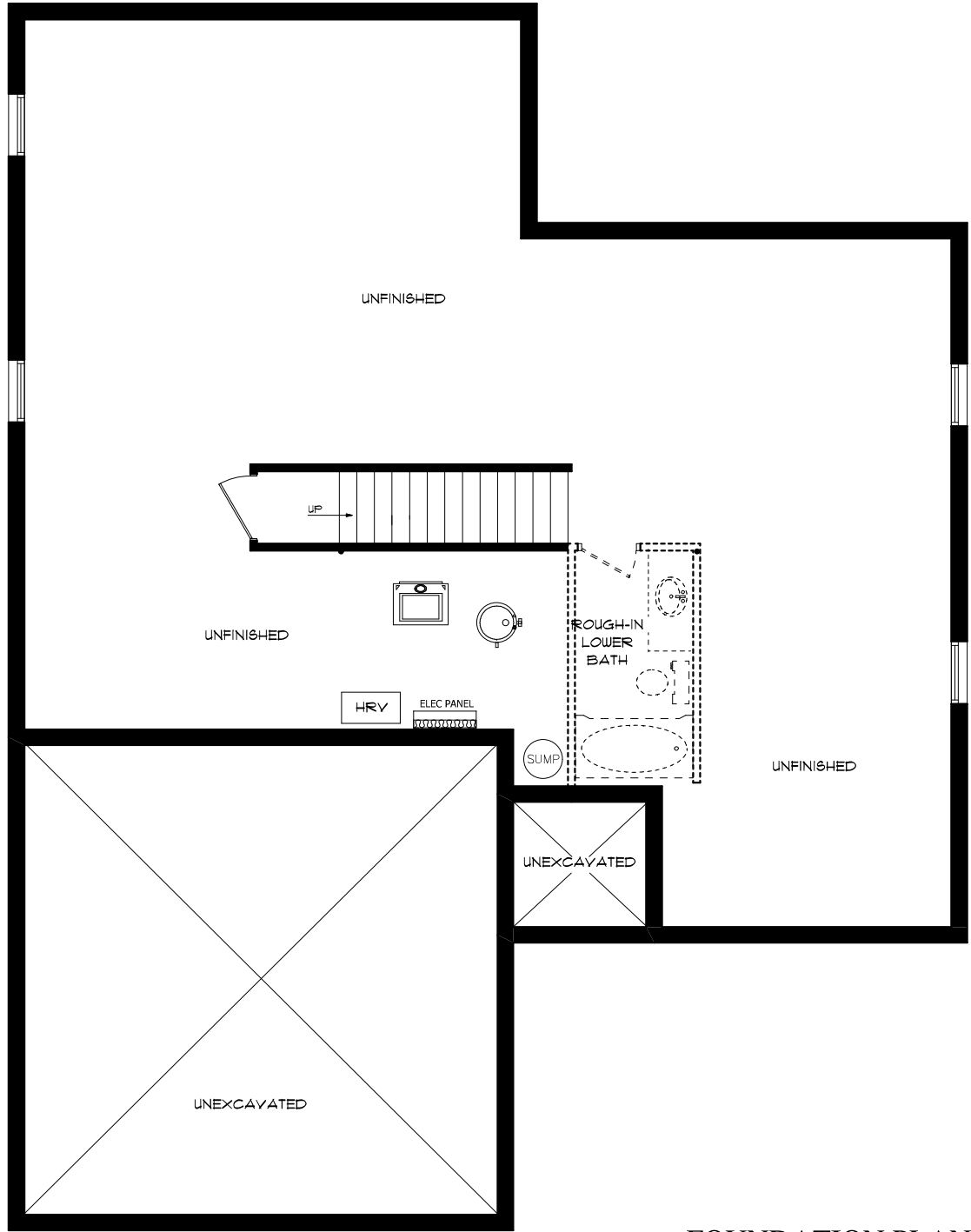
FOUNDATION PLAN
