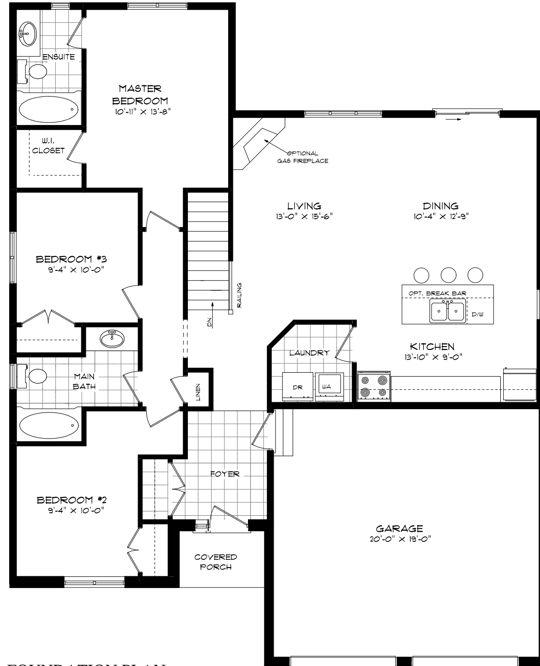
FOUNDATION PLAN
