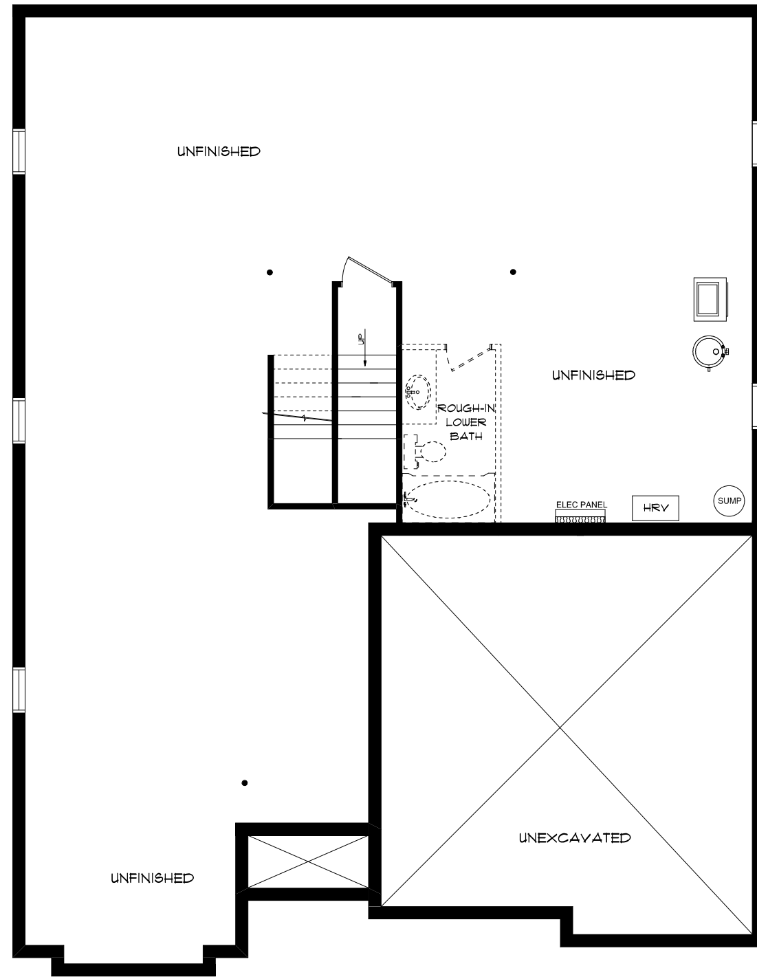
FOUNDATION PLAN
