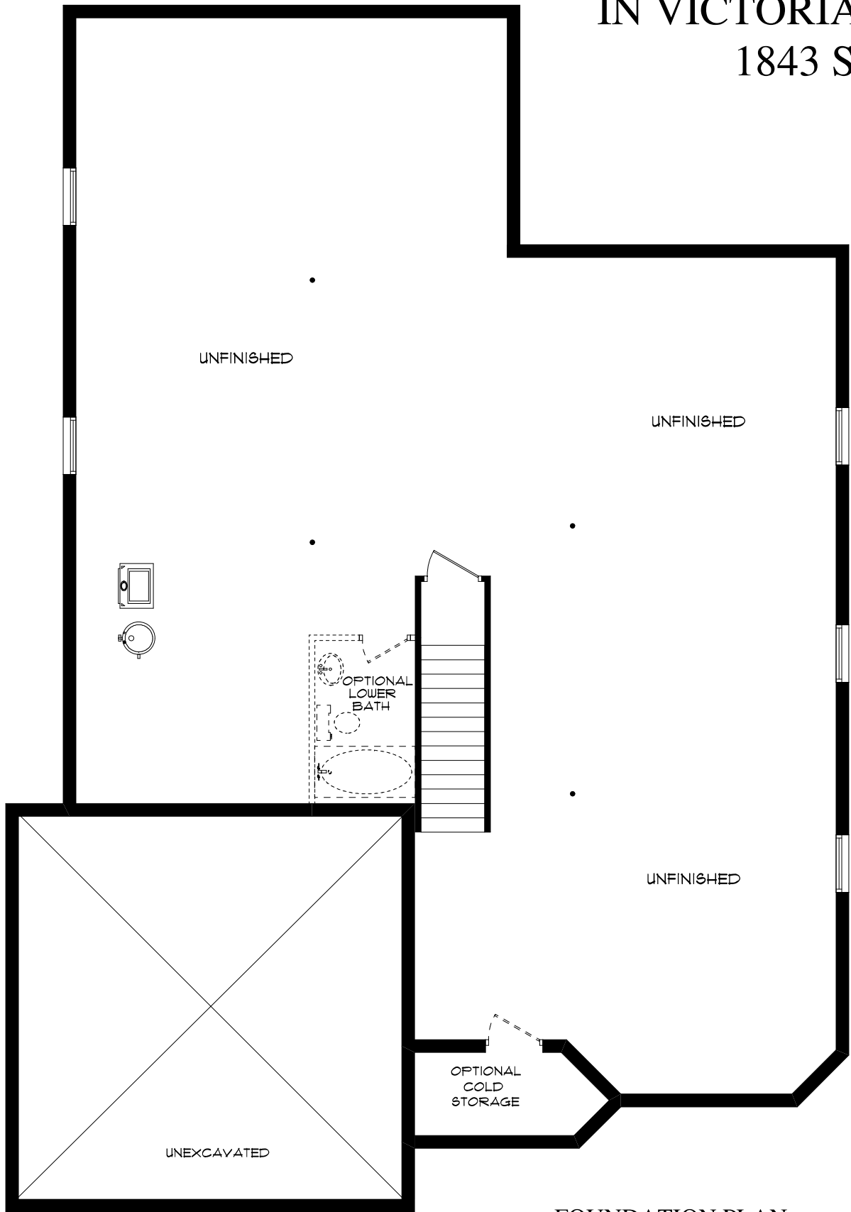
FOUNDATION PLAN
